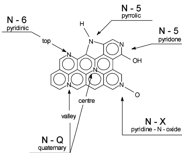
Fig. 15 Bonding configurations for nitrogen atoms in carbon materials. Reproduced with permission from ref. 106. Copyright © 2003 Elsevier Science Ltd.
