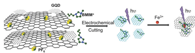
Fig. 2 Schematic illustration of GD synthesis from 3D graphene and the mechanism of \text{Fe}^{3+} detection. Reprinted with permission from ref. 42. Copyright (2014) Wiley-VCH Verlag GmbH & Co. KGaA, Weinheim.
