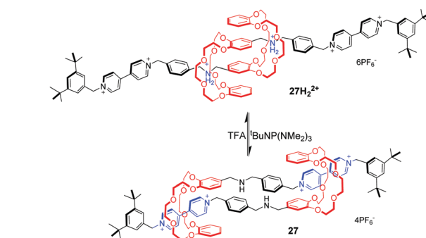
Fig. 27 pH-Actuated [c2]daisy chain 27 .
