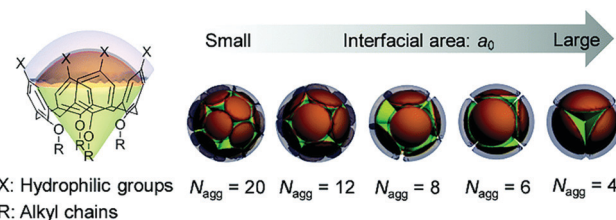
Fig. 4 Chemical structure of a calix[4]arene-based amphiphile and the schematic illustration of the effect of the size of interfacial area on the N_{\text{agg}} of the micelles composed of the amphiphiles. Reprinted with permission from ref. 65. Copyright 2018 from Royal Society of Chemistry.
