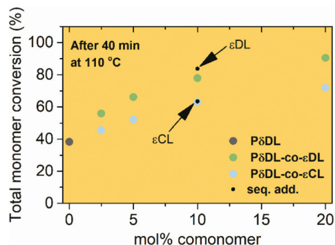
Fig. 5 The plot shows how the total monomer conversion of \text{P}\delta\text{DL-co-}\epsilon\text{DL} (green) and \text{P}\delta\text{DL-co-}\epsilon\text{CL} (blue) depends on the feed mol% of the comonomer after 40 min at 110 °C. The circles represent one-step copolymerization and the black points represent copolymerization by sequential addition. The grey circle represents \delta DL homopolymer.
