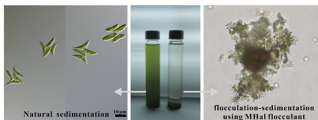
Fig. 7 Amine-modified HNTs induce rapid flocculation and sedimentation of the microalgae Scenedesmus dimorphus . Light microscope images of the freshwater microalgae with APTES-modified HNTs (termed as MHaI, right panel) and without HNTs (left panel). Positively charged APTES-HNTs co-aggregate with negatively charged microalgae cells causing subsequent flocculation and sedimentation significantly shortening the harvest process. Reproduced from ref. 135. Copyright 2019, with permission from Elsevier.
