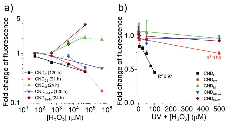
Fig. 6 Oxidation dependent fluorescence of CNDs. (a) Concentration-dependent change of fluorescence emission of CNDs in the presence of H 2 O 2 (log–log scale) for a duration indicated between parentheses in the legend ( \lambda_{\text{ex}} 360 nm; \lambda_{\text{em}} is the maximum emission wavelength seen in preceding figures). R^2 was 0.96–0.99 for all linear fits. (b) Concentration-dependent change of fluorescence emission of CNDs (linear scale) after 30 min exposure to H 2 O 2 and UV radiation to produce hydroxyl radicals. For both panes, data presented as mean + SD, n = 3 .
