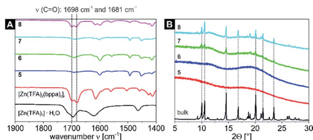
Fig. 3 Detailed view on the spectral range of 1900\text{ cm}^{-1} to 1400\text{ cm}^{-1} of the IR spectra of the starting material [\text{Zn}(\text{TFA})_2] \cdot \text{H}_2\text{O} , the CN [\text{Zn}(\text{TFA})_2(\text{bppa})_2]_n and the four [\text{Zn}(\text{TFA})_2(\text{bppa})_2]_n nanocomposite samples 5–8 (A). The complete spectra can be found in Fig. S8†. Comparison of the PXRD patterns of the bulk material [\text{Zn}(\text{TFA})_2(\text{bppa})_2]_n and the [\text{Zn}(\text{TFA})_2(\text{bppa})_2]_n nanocomposite samples 5–8 (B). Most intense PXRD reflexes that correlate with the bulk material are marked with a dashed line.
