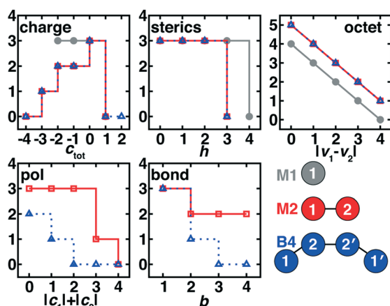
Fig. 2 Scores for each of the three ligand types (i.e., M1 in gray circles and solid lines, M2 in red squares and solid lines, and B4 in blue triangles and dotted lines) colored according to the bottom right inset. Three of the scores apply to all three ligand types: charge ( c_{\text{tot}} , top left); sterics, as judged through number of hydrogen atoms on the metal-coordinating atom ( h , top middle); and octet, as judged through valence deviations ( |v_1 - v_2| , where v_2 = 8 for M1 ligands, top right). Two of the scores apply only to M2 and B4 ligands: pol, the polarization measured by |c_1| + |c_2| (bottom, left) and bond, b , for the 1–2 bond order (bottom, middle).
