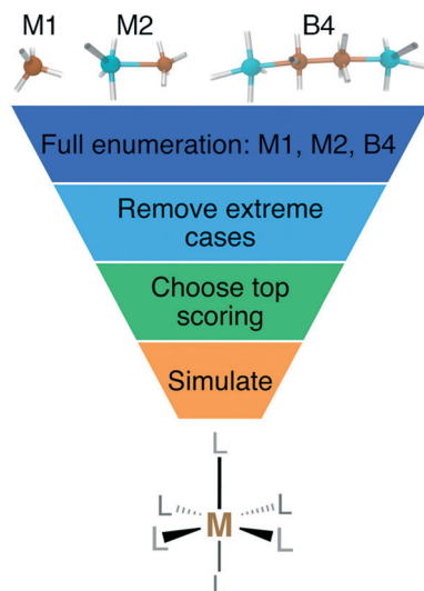
Fig. 1 Schematic of M1, M2, and B4 ligands, as designated by the number of heavy atoms (i.e., C, N, O, P, or S) and number of metal-coordinating atoms (top) with hypothetical places to add hydrogen atoms indicated with white sticks. The filtering process consists first of enumeration of all possible ligands, removal of extreme cases, scoring and retaining top-scoring ligands, and then finally the simulation of homoleptic M_{(II)}/M_{(III)} ( M = \text{Cr, Mn, Fe, or Co} ) octahedral complexes with DFT as indicated in the flowchart.
