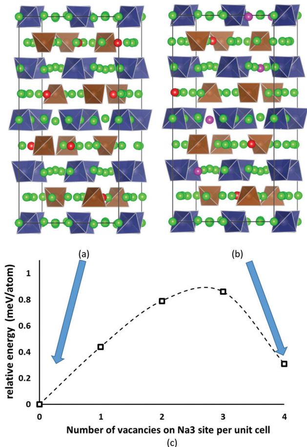
Fig. 2 The two lowest energy configurations for \text{Na}_{11}\text{Sn}_2\text{PS}_{12} : (a) the lowest energy configuration containing 8 vacancies on Na2 (32g) sites, (b) the second-lowest energy configuration with the Na/vacancy distribution previously reported by Yu et al. 47 containing four vacancies on Na2 (32g) sites and four on Na3 (16d) sites. Grey (brown) tetrahedra represent \text{SnS}_4 ( \text{PS}_4 ), green spheres occupied Na sites, while Na2 (Na3) vacancies are marked in red (magenta). (c) Energy profile for the lowest energy interconversion between these two configurations.
