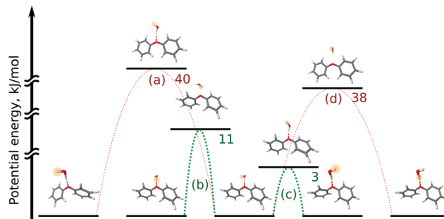
Fig. 8 Scheme for motions in the OH-O DPE-( \text{H}_2\text{O} ) isomer that inter-connect equivalent minima on the PES. This scheme contains a set of five equivalent minima and the transition states that lead from the central minimum to others. The letters in parentheses denote the motion (see text for details), numbers denote the transition state energies in \text{kJ mol}^{-1} computed at the DLPNO-CCSD(T)/def2-TZVPP//B97-3c level of theory. The yellow highlighting and its absence indicate the positions of the unique protons.
