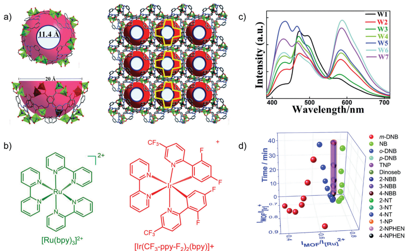
Fig. 9 (a) Structure of Zn-MOF [DMA] 2 [Zn 2 (L)(H 2 O)] with the aperture and cage sizes. (b) Structures of [Ru(bpy) 3 ] 2+ and [Ir(CF 3 -ppy-F) 2 (bpy)] + . (c) Emission spectra ( \lambda_{\text{ex}} = 365 nm) for loading different amounts of Ir- and Ru-complex guests in the Zn-MOF. W1: 0.88/0.55 wt% Ir/Ru complex; W2: 0.28/0.45; W3: 0.18/0.25; W4: 0.18/0.46; W5: 0.13/0.35; W6: 0.065/0.46; W7: 0.065/0.42. (d) Derived 3D ratiometric sensing of nitroaromatic vapors with signal evolution time as the third dimension. Reproduced from ref. 78 with permission from the Royal Society of Chemistry, copyright 2018.
