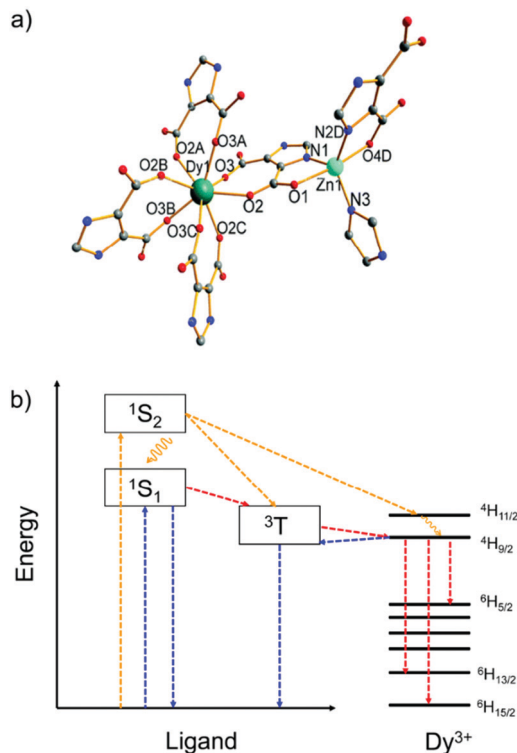
Fig. 1 (a) Coordination environments of Zn 2+ and Dy 3+ in the MOF [H(H 2 O) 8 ][DyZn 4 (imdc) 4 (im) 4 ]. (b) Energy level diagram of the yellow and white light emission from the Zn 2+ /Dy 3+ -MOF. Color scheme: yellow, pathways for excitation at 290 nm; blue, pathways for excitation at 340 nm; red, pathways for excitation at both 290 and 340 nm. Reproduced from ref. 43 with permission from the Royal Society of Chemistry, copyright 2016.
