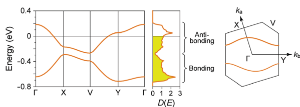
Fig. 15 Electronic band dispersions, densities of states ( D(E) in states per electronvolt per spin), and Fermi surfaces of (\text{TMTTF})_2\text{PF}_6 , calculated on the basis of the extended Hückel method with the tight-binding approximation using crystallographic data at room temperature. The energy is provided relative to the Fermi energy. Note that the electron–electron correlation is not considered in this calculation.
