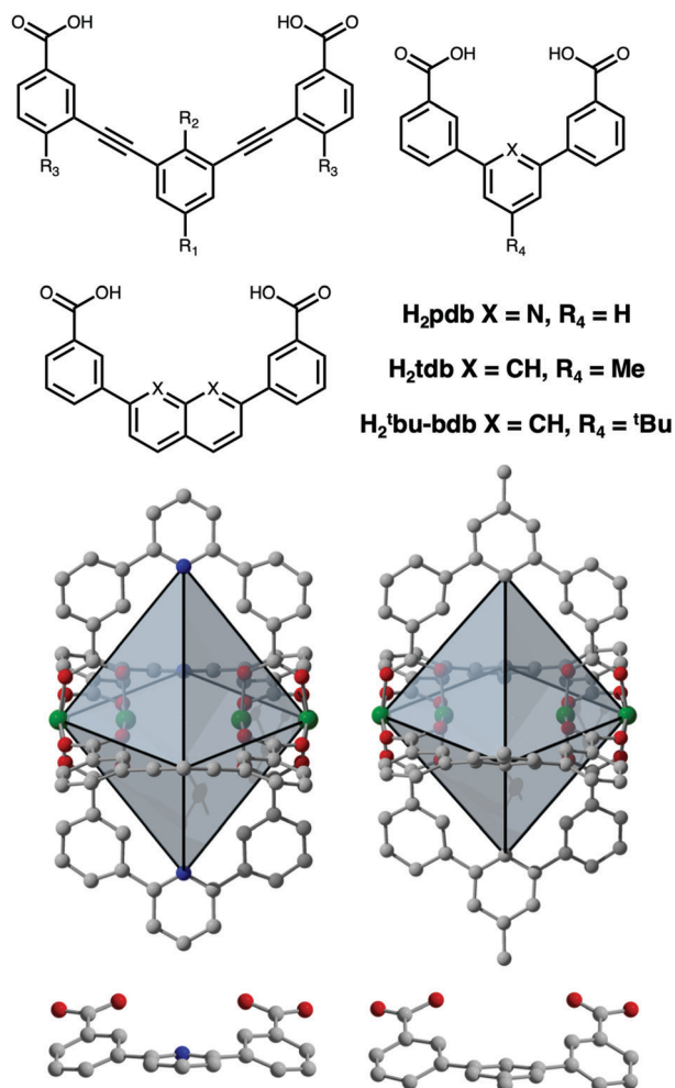
Fig. 1 (Top Left) Prominent ligands for porous lantern-type paddlewheel cages that have been combined with Cu, Mo, or Rh to afford M_4L_4 structures. This study focuses on Cu_4(pdb)_4 , Cu_4(^tBu-bdb)_4 , and M_4(tdb)_4 where M = Cr, Cu, Mo . (Bottom) Structures of Cu_4(pdb)_4 (left) and Cu_4(tdb)_4 (right) where green, red, gray, and blue spheres represent copper, oxygen, carbon, and nitrogen atoms, respectively. Although the pyridine-based cage has no C–H on the central ring, the ligand is significantly distorted away from planarity in the crystal structure.
