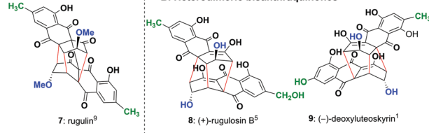
Fig. 1 (A) Homodimeric bisanthraquinones 1–5 and 7 isolated from various fungal species and not yet isolated analogue 6 and (B) heterodimeric bisanthraquinones 8 and 9 isolated from fungi.
