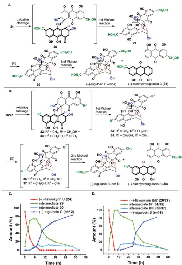
Scheme 4 (A) Cascade conversion of (–)-flavoskyrin C ( 24 ) to (–)-rugulosin C ( ent - 2 ). (B) Cascade conversion of (–)-flavoskyrin B/B' ( 26/27 ) to (–)-rugulosin B ( ent - 8 ). (C) Plot of percentage conversion of the products formed with time (h) for the cascade in (A). (D) Plot of percentage conversion of the products formed with time (h) for the cascade in (B).
