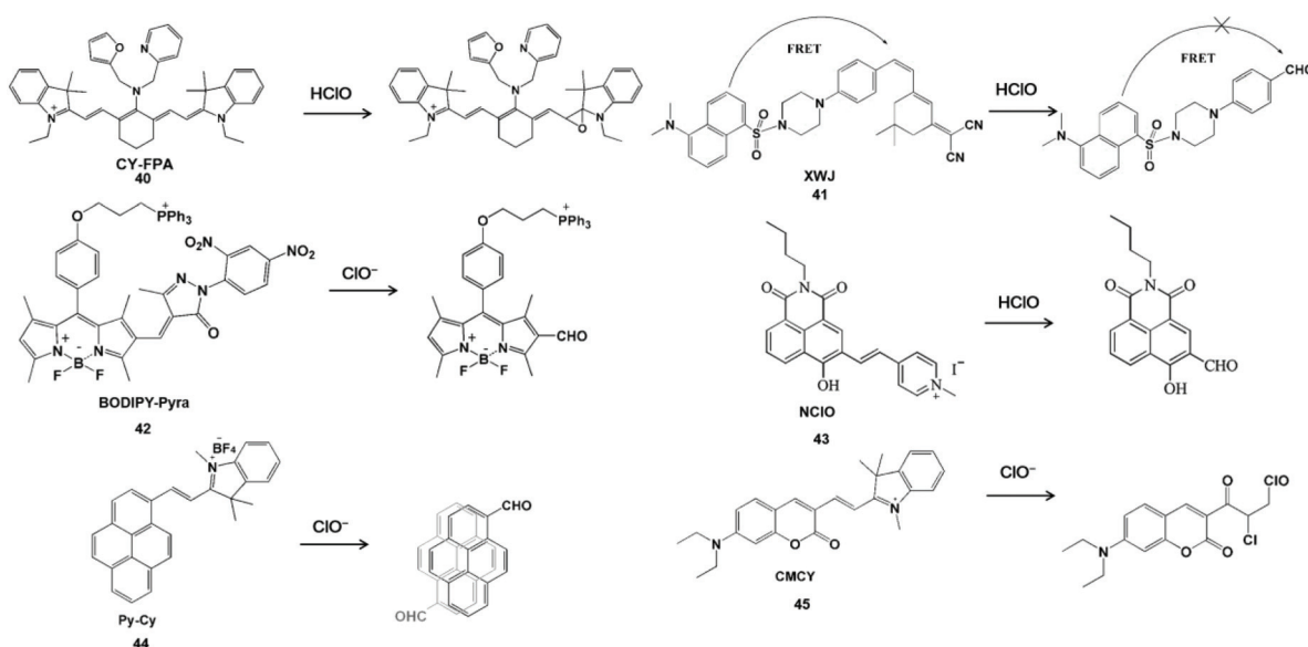
Scheme 10 Structures and mechanism of C=C unsaturated double bonds for HClO/HClO - probes. Reprinted with permission from ref. 92. Copyright 2014, American Chemical Society. Reprinted with permission from ref. 94. Copyright 2014, American Chemical Society. Reprinted with permission from ref. 97. Copyright 2019, Elsevier. Reprinted with permission from ref. 98. Copyright 2019, Elsevier. Reprinted with permission from ref. 99. Copyright 2016, American Chemical Society. Reprinted with permission from ref. 100. Copyright 2014, Royal Society of Chemistry.
