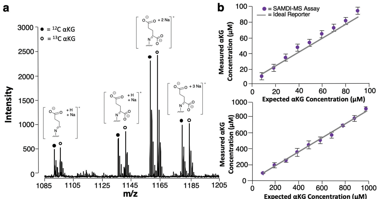
Fig. 3 (a) Representative SAMDI-MS spectrum of a 1 mM 12 C and 1 mM 13 C \alpha KG solution displaying the sodium adduct of the \alpha -cleavage product at m/z = 1091 ( 12 C) and m/z = 1095 ( 13 C), the sodium adduct at m/z = 1135 ( 12 C) and m/z = 1140 ( 13 C), the double sodium adduct at m/z = 1157 ( 12 C) and m/z = 1162 ( 13 C) and the triple sodium adduct at m/z = 1179 ( 12 C) and m/z = 1184 ( 13 C). (b) Sensitivity plots comparing measured \alpha KG concentration to known \alpha KG concentration for solutions ranging from 10 to 90 \mu M (top) and from 100 \mu M to 1 mM (bottom). Data are expressed as mean \pm standard deviation, with n = 8 –10 technical replicates per solution.
