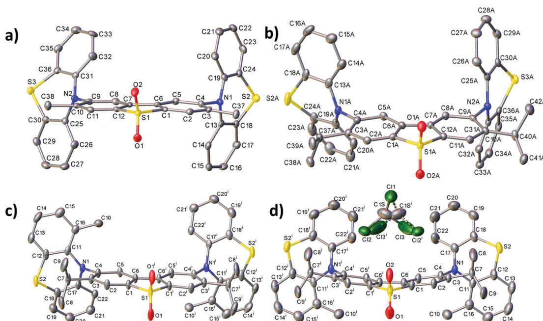
Fig. 2 Molecular structures of 6 (a), 7 at 120 K (b), 8 (c) and 8 -CDCl 3 (d) showing ellipsoids at 50% probability. H atoms are omitted. Primed atoms are generated by a twofold axis (c) and a mirror plane (d).
