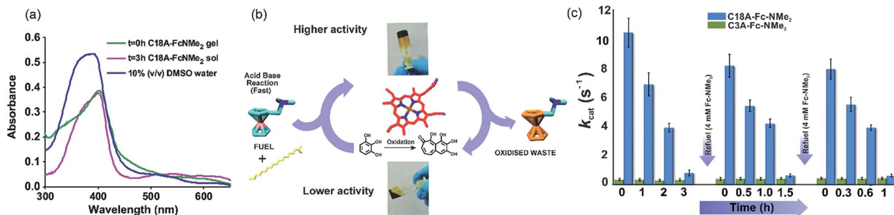
Fig. 4 (a) UV-vis spectra of free hemin and hemin entrapped C18A-FcNMe 2 gel at \approx 0 h and 3 h. All samples had histidine (1 mM). (b) Schematic representation of the temporal regulation of artificial peroxidase activity of hemin entrapped in the transient system. (c) k_{\text{cat}} values of hemin (0.1 mM) catalyzed oxidation of pyrogallol (varying concentration) by H 2 O 2 (30 mM) in the presence of 1 mM histidine for C18A-FcNMe 2 and C3A-FcNMe 2 systems. The error bars are the result of triplicate measurements.
