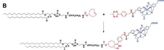
Fig. 4 (A) Radio-HPLC chromatograms of (top) ^{68}\text{Ga} ]-Ga-HBED-CC-tetrazine precursor and (bottom) reaction between 4 and 5, after 15 min at 60 ^{\circ}\text{C} . (B) Scheme of the reaction between TCO-modified PE (4) and ^{68}\text{Ga} ]-Ga-HBED-CC-tetrazine (5).
