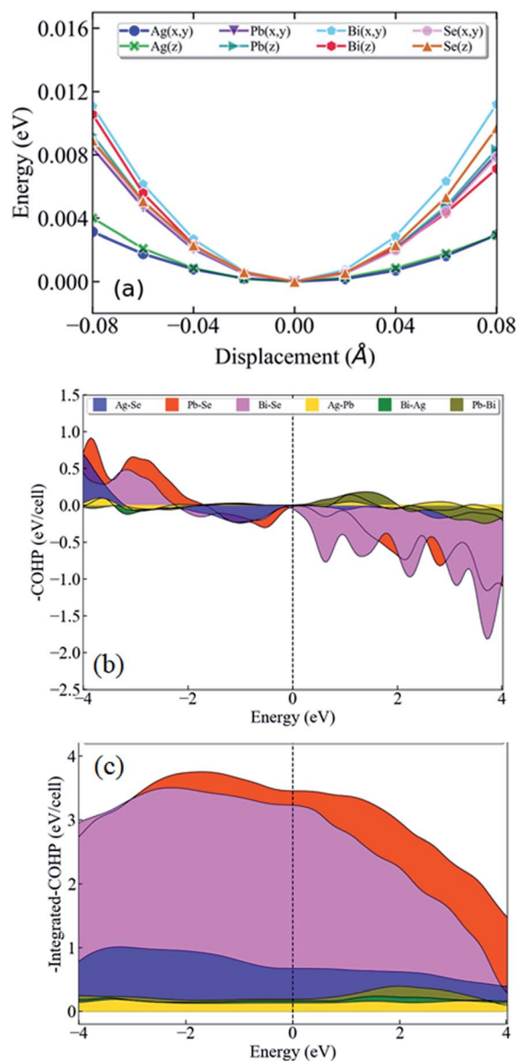
Fig. 3 (a) Potential energy curves of the constituent atoms in AgPbBiSe 3 as a function of displacement around their equilibrium positions along the x - and z -direction. (b) Crystal orbital Hamiltonian population (COHP) and (c) integrated COHP (iCOHP) for the nearest neighbor atomic pairs of AgPbBiSe 3 . The smaller peak in (b) below the Fermi level and smallest area under the curve in (c) of Ag–Se interaction shows that the Ag atoms have the weakest bonding to the lattice.
