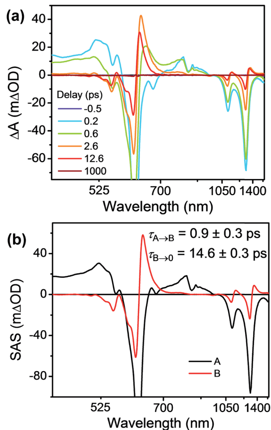
Fig. 6 (a) fsTA spectra and (b) species-associated spectra (SAS) of Bn-TTz 2+ in CH 3 CN excited at 620 nm ((A) 2* TTz 2+ (D n ), (B) 2* TTz 2+ (D 1 )). The wavelength axis is plotted in reciprocal space. Time constants are for the representative data set shown here; averages and standard deviations from multiple experiments are given in Table 1.
