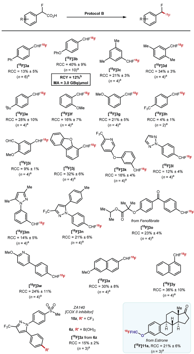
Scheme 5 Scope of [ ^{18}\text{F} ]fluorodecarboxylation applying protocol B: ^{\text{a}}\text{ArCHFCO}_2\text{H} (0.028 mmol), PhIO (0.5 equiv.), MeCN (1 mL), 50 ^{\circ}\text{C} , 10 min then addition of [ ^{18}\text{F} ]TEAF (20–30 MBq) Mn(tmp)Cl (2 mg), DMF (300 \mu L), 50 ^{\circ}\text{C} , 20 min. ^{\text{b}}\text{ArCHFCO}_2\text{H} (0.014 mmol), PhIO (0.5 equiv.), MeCN (1 mL), 50 ^{\circ}\text{C} , 10 min then addition of [ ^{18}\text{F} ]Mn(tmp)F (841 MBq) DCE (300 \mu L), 60 ^{\circ}\text{C} , 20 min.
