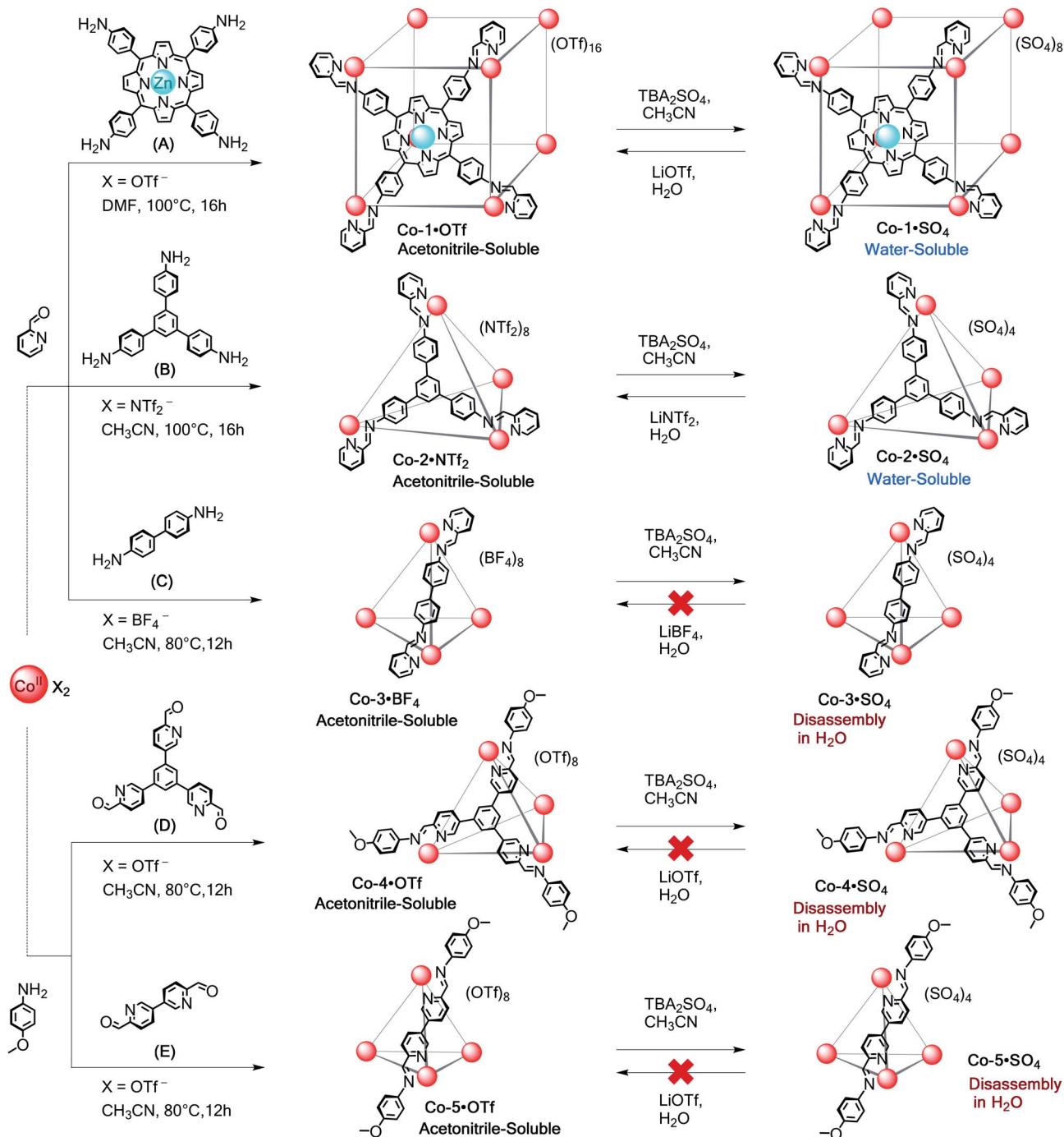
Scheme 1 Subcomponent self-assembly of Co II -capsules. Preparation of acetonitrile-soluble Co-1•X to Co-5•X (X = OTf - , NTf 2 - , or BF 4 - ) from subcomponents A–E and their anion exchange sequences.
