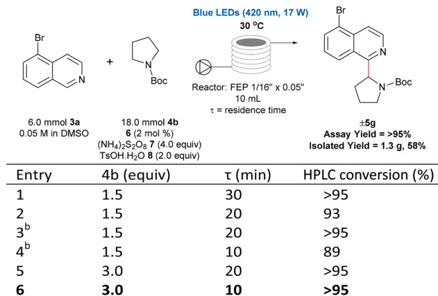
a Percent conversion based on relative HPLC peak area integrations of starting material compared with product. b 4 mol % of photocatalyst 6 [ \text{Ir}(\text{dF}(\text{CF}_3)\text{ppy})_2(\text{dtbpy})\text{PF}_6 ].
