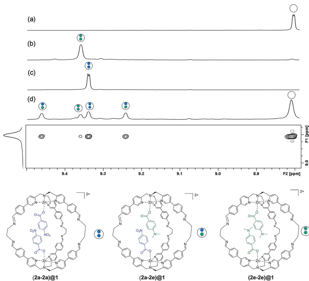
Fig. 3 Partial 500 MHz 1 H NMR spectra showing the signals due to the cage pyridine \alpha protons (301 K, CD 3 CN) for (a) cage 1 (b) (2e-2e)@1 (c) (2a-2a)@1 and (d) 1 H ROESY experiment for the competition experiment between guest 2a and 2e ([ 1 ] = 1.0 mM, [ 2a ] = [ 2e ] = 0.1 mM). Counterions are perchlorate for the cage and triethyl ammonium for the guest and they are omitted for clarity.
