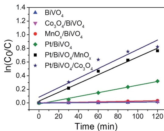
Fig. 6 Kinetic fitting of the CBZ degradation on different photocatalysts. Reaction conditions: 100 mL CBZ solution with initial concentration of 10 \text{ mg L}^{-1} , catalyst dosage 1 \text{ g L}^{-1} , the contents of the deposited Pt is 0.2 wt%, \text{Co}_3\text{O}_4 and \text{MnO}_x are all 0.1 wt% and 300 W Xe lamp ( \lambda > 420 \text{ nm} ), top irradiation.
