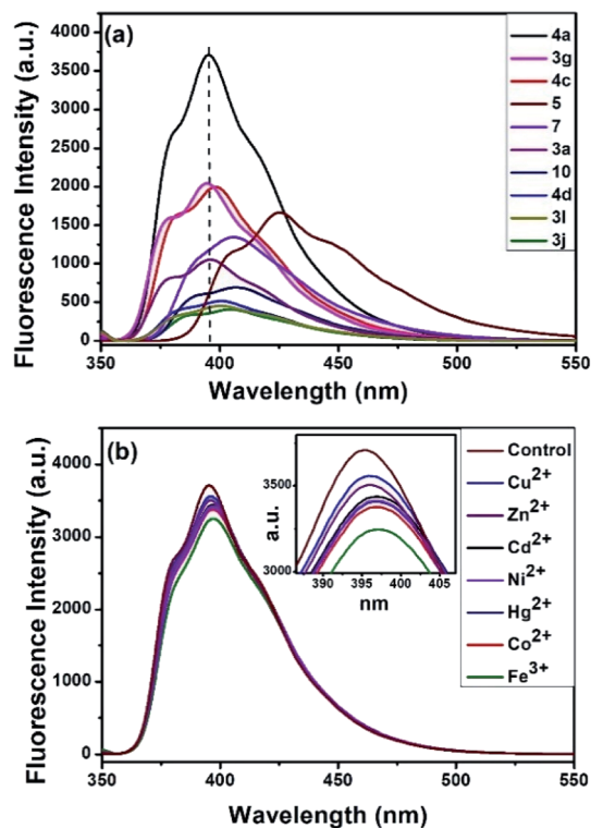
Fig. 3 (a) Fluorescence responses of different compounds (10 \mu\text{M} , \lambda_{\text{ex}} = 350 nm). (b) Fluorescence responses of 4a in the presence of various metal cations (10 \mu\text{M} , \lambda_{\text{ex}} = 350 nm).
