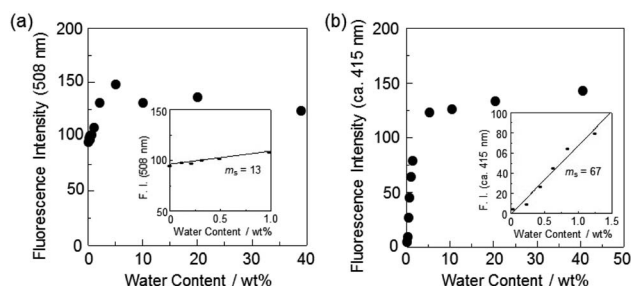
Fig. 5 Fluorescence peak intensity at (a) 508 nm of DJ-1 ( \lambda^{ex} = 367 nm) and (b) around 415 nm of OM-1 ( \lambda^{ex} = 366 nm) as a function of water content below 40 wt% in acetonitrile. Inset in (a): fluorescence peak intensity at 508 nm of DJ-1 ( \lambda^{ex} = 367 nm) as a function of water content below 1.0 wt% in acetonitrile. Inset in (b): fluorescence peak intensity at around 415 nm of OM-1 ( \lambda^{ex} = 366 nm) as a function of water content below 1.3 wt% in acetonitrile.
