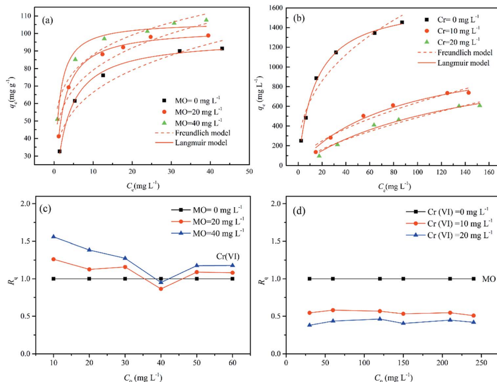
Fig. 6 Adsorption isotherms of Cr(vi) (a) and MO (b) by MWCNTs@Fe 3 O 4 /PEI in MO-Cr(vi) binary system. (Conditions: initial dye concentration, 30–240 \text{mg L}^{-1} for MO, 10–60 \text{mg L}^{-1} for Cr(vi); adsorbent dosage, 3 mg for MO, 10 mg for Cr(vi); solution pH, 3; contact time, 6 h for MO, 4 h for Cr(vi); temperature, 25–55 ^{\circ}\text{C} ; and agitation speed, 150 rpm.)
