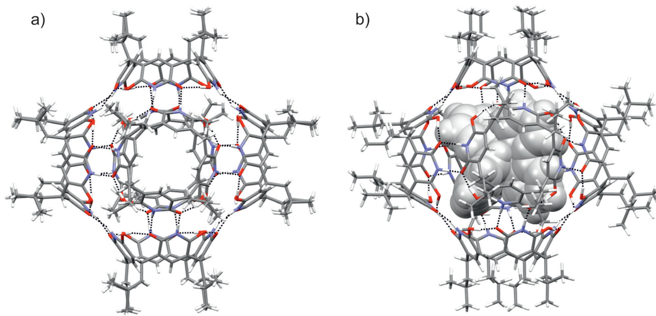
Fig. 3 X-Ray crystal structure of 1 6 and (b) optimized structure of [ 1 6 + G ] 2+ at the RI-PBE-D3/def2-SVP level of theory in capped stick model. Tris (bipyridine)-ruthenium(II) ( G ) is shown in grey CPK model in (b). Black dashed lines represent hydrogen bonds. Color code: H = white, C = grey, N = blue, O = red.
