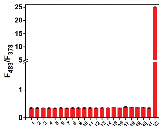
Fig. 2 Fluorescence intensity ratio changes (based on the peak heights at the maxima, 378 and 483 nm respectively) with addition of \text{O}_2^{\bullet-} (39 equiv.) and other interfering reagents (120 \mu\text{M} ). 1. Probe only; 2. \text{ClO}^- ; 3. \text{H}_2\text{O}_2 ; 4. \cdot\text{OH} ; 5. ^1\text{O}_2 ; 6. \text{ONOO}^- ; 7. \text{ROO}\cdot ; 8. \text{H}_2\text{S} ; 9. glucose; 10. GSH; 11. Cys; 12. Hcy; 13. \text{Na}^+ ; 14. \text{K}^+ ; 15. \text{Ca}^{2+} ; 16. \text{Mg}^{2+} ; 17. \text{Zn}^{2+} ; 18. \text{Fe}^{2+} ; 19. \text{Al}^{3+} ; 20. \text{Cu}^{2+} ; 21. \text{Fe}^{3+} ; 22. \text{O}_2^{\bullet-} . \lambda_{\text{ex}} = 310 nm. Error bar represents s.d. Slit widths: ex = 8 nm, em = 5 nm. 30 min wait between measurements.
