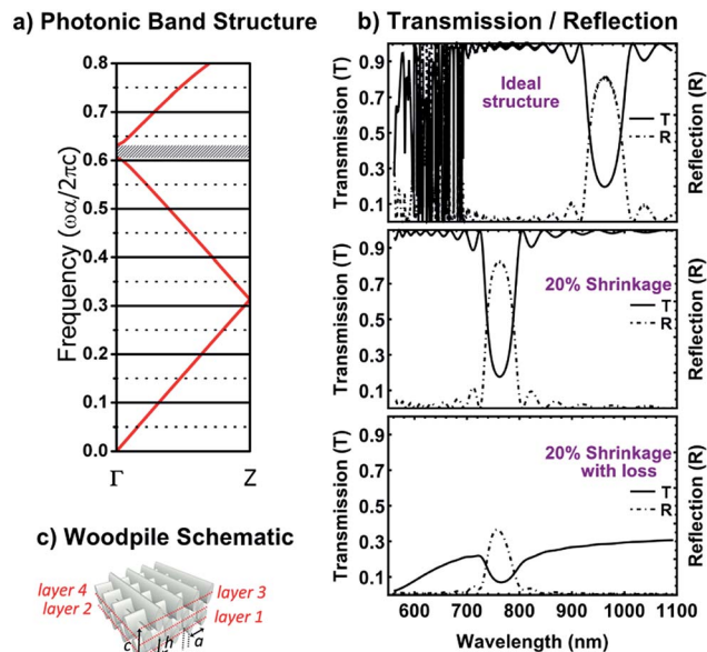
Fig. 6 Theoretical calculations along the stacking direction ( \Gamma Z) of a woodpile photonic crystal with an inlayer periodicity a = 600 nm: (a) photonic band structure calculations of infinite system, (b) simulated transmission (solid) and reflection (dashed-dot) response for finite system with 10 unit cells ( 4 \times 10 = 40 layers), which is assumed to be infinite in the inlayer plane; (i) ideal structure (upper panel), (ii) introducing 20% shrinkage to the ideal structure (middle panel), (iii) introducing artificial loss (conductivity, \sigma ) into the dielectric rods of the shrunken structure equal to \sigma = 3 \times 10^{-3} S (lower panel), and (c) schematic of the woodpile photonic crystal showing one unit cell (of length c ) along the stacking direction.
