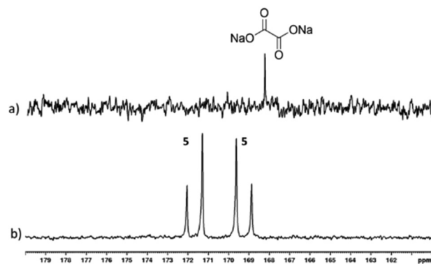
Fig. 4 (a) 128 scan ^{13}\text{C} spectrum of a solution of 1 , DMSO and sodium-1,2-oxalate- [\text{C}_2^{13}] (1 : 5 : 5) in methanol- d_4 (b) ^{13}\text{C} NMR signals seen after shaking an NMR tube with 3-bar p\text{-H}_2 in a mu metal shield for 30 seconds.
