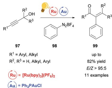
Scheme 37 Tandem arylation Meyer–Schuster rearrangement. Reagents and conditions: propargyl alcohol (1.00 equiv.), PhN 2 BF 4 98 (4.00 equiv.), KH 2 PO 4 (4.00 equiv.), Ru-photocat. (2.5 mol%), Au-cat. (10.0 mol%), MeOH, rt, Ar, 5 W green LED, 16 h. 123,126
