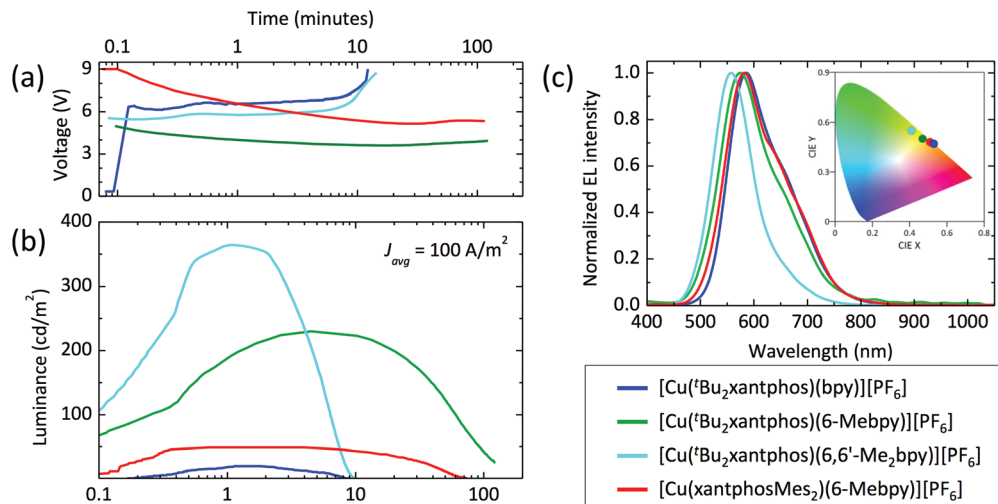
Fig. 14 Time evolution of the (a) voltage and (b) the luminance for a series of LECs driven at an average current density of 100 \text{ A m}^{-2} . (c) Electroluminescence spectra for the same device series with (inset) the corresponding colour coordinates in the CIE 1931 colour space.
