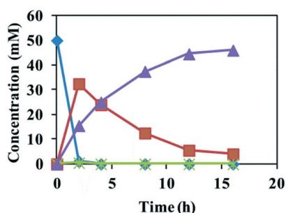
Fig. 1 Time course of the conversion of styrene oxide 1c (50 mM) to ( S )- 4c with resting cells of E. coli (SpEH-BDHA-GoSCR-MVTA) (20 g cdw L -1 ) in a two-liquid phase system. \blacklozenge = the concentration of 1c ; \blacksquare = the concentration of 2c ; \otimes = the concentration of 3c ; and \blacktriangle = the concentration of ( S )- 4c .
