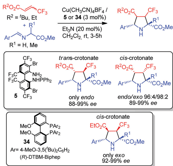
Scheme 15 \text{Cu}^{\text{I}} /( S )-TF-BiphamPhos catalyzed cycloaddition with trifluorocrotonates.
