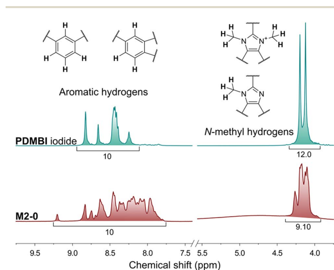
Fig. 5 1 H NMR spectra of PDMBI iodide and M2-0 membrane showing aromatic and N -methyl hydrogens. The area ratios of the signals show 100% and 50–60% quarternisation of the benzimidazole groups for PDMBI and M2-0 , respectively.
