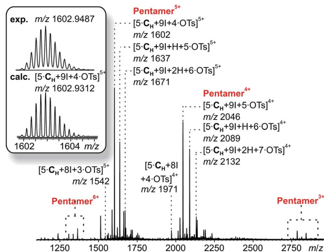
Fig. 5 ESI-Q-TOF-HRMS spectrum of pentameric halogen-bonded capsule 3 (90 \mu M in \text{CH}_2\text{Cl}_2 ) with experimental and calculated isotopic pattern (inset).
