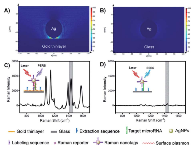
Fig. 2 Electric-field intensity simulated by FDTD under (A) PERS mode and (B) SERS mode. Representative Raman spectra for (C) PERS mode and (D) SERS mode. Insertions show schematic of the principle of PERS and SERS modes.
