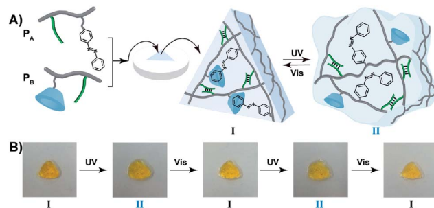
Fig. 2 (A) Schematic preparation of a triangle-shaped CMC hydrogel crosslinked by the (1)/(1) duplexes and \beta -azobenzene/ \beta -CD complexes, and light-induced reversible transitions between the stiff shaped hydrogel I and the shapeless quasi-liquid hydrogel II that is only crosslinked by the (1)/(1) bridges. (B) Macroscopic images of the reversible light-induced transitions of the hydrogel between the triangle-shaped hydrogel I and the quasi-liquid shapeless hydrogel II, respectively.
