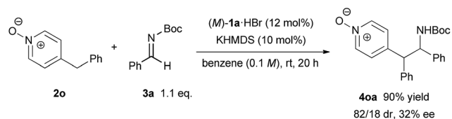
Scheme 4 Control experiment.
