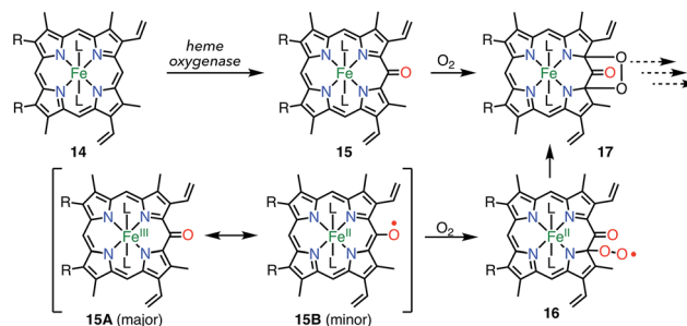
Fig. 7 Heme catabolism.
