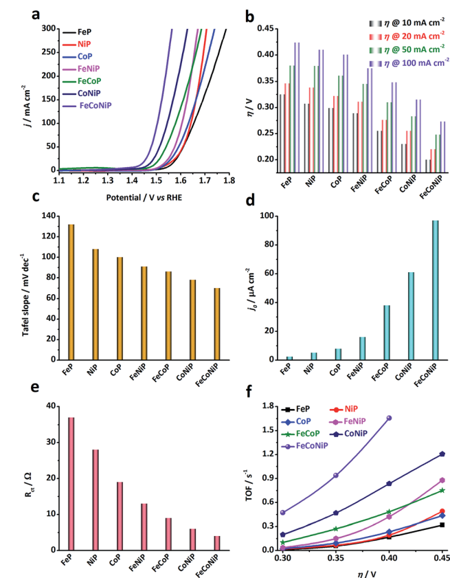
Fig. 2 OER performance of different TMP pre-catalysts measured in 1.0 M \text{O}_2 -saturated KOH electrolyte. (a) iR -corrected polarization curves ( i.e. the cathodic branches of the CV curves shown in Fig. S10, ESI†) of the TMP pre-catalysts, recorded at a scan rate of 5 \text{mV s}^{-1} in the potential range of 1.0 to 1.8 V vs. RHE. (b) The overpotentials needed to deliver anodic current densities of 10, 20, 50 and 100 \text{mA cm}^{-2} for all TMP pre-catalysts. (c) Tafel slopes, (d) exchange current densities, and (e) charge transfer resistance ( R_{ct} ) values measured at 1.45 V vs. RHE. (f) TOF values calculated at \eta = 300, 350, 400 and 450 mV.
