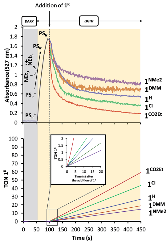
Fig. 8 (Top) UV-Vis spectral changes monitored at 527 nm associated with the formation of \text{PSIr} upon irradiation at \lambda = 447 nm and addition of \mathbf{1}^{\text{R}} complexes (0.1 eq. vs. \text{PSIr}^+ ). (Bottom) Time-dependent photocatalytic \text{H}_2 evolution during the first seconds after addition of \mathbf{1}^{\text{R}} . Inset: magnification of the \text{H}_2 evolution during the first seconds after addition of \mathbf{1}^{\text{R}} . Conditions: [\text{PSIr}^+] = 0.25 mM, [\text{Et}_3\text{N}] = 100 mM, \text{CH}_3\text{CN} : \text{H}_2\text{O} (0.8 : 1.2 mL) at 25 °C.
