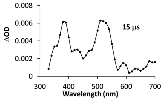
Fig. 9 Transient absorption spectrum of a solution containing \text{PSIr}^+ (50 \mu\text{M} ), \text{Et}_3\text{N} (20 mM) and \mathbf{1}^{\text{CO}_2\text{Et}} (80 \mu\text{M} ) recorded at 15 \mu\text{s} after laser excitation. All measurements were carried out under \text{N}_2 at room temperature in acetonitrile ( \lambda_{\text{ex}} = 355 nm, E = 8 mJ per pulse).
