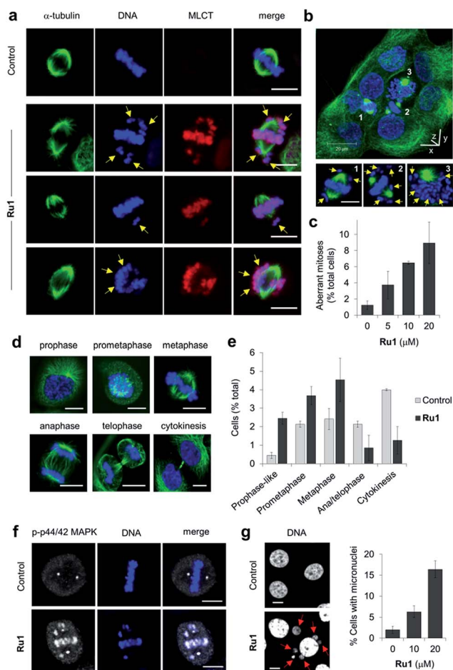
Fig. 4 (a) Misaligned metaphase chromosomes (yellow arrows) in OE21 cells treated with Ru1 (20 \mu M, 4 h). After fixation, cells were stained for \alpha -tubulin (green) and DNA (DAPI, blue). MLCT (metal to ligand charge-transfer) emission of Ru1 included. (b) 3D representation of Ru1 -treated OE21 cells (20 \mu M, 24 h) prepared from z-stack images. Non-aligned chromosomes in labelled cells shown by yellow arrows. (c) Quantification of aberrant mitoses in Ru1 -treated OE21 cells (24 h). Data average of two independent experiments \pm S.D., >200 cells were counted for each condition. (d) CLSM images of mitotic stages of OE21 cells. (e) Quantification of mitotic sub-populations in Ru1 -treated OE21 cells (20 \mu M, 24 h). Data are expressed as a percentage of total cell population. Data average of two independent experiments \pm S.D., >200 cells counted per experiment. (f) Localisation of phospho(p)-p44/p42 MAP kinase in metaphase OE21 cells treated with Ru1 (20 \mu M, 24 h), as determined by immunofluorescence (AlexaFluor594, white). DNA staining (DAPI, blue) included for reference. (g) Formation of micronuclei (red arrows) in OE21 cells treated with Ru1 (20 \mu M, 24 h). Data average of two independent experiments \pm S.D. where >100 cells were counted for each condition. Scale bars = 10 \mu m.
