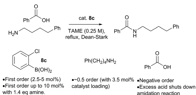
Scheme 12 Preliminary kinetics studies on a boronic acid catalyzed amidation reaction.
