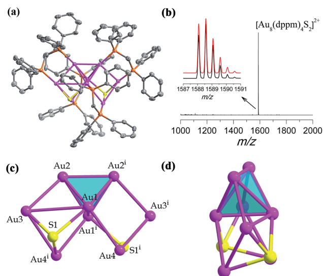
Fig. 2 (a) The X-ray crystal structure of cationic [Au 8 (dppm) 4 S 2 ] 2+ . Thermal contours are drawn at the 50% probability level. Color labels: purple, Au; orange, P; and gray, C. H atoms and Cl − ions are omitted. (b) The positive mode of the HRESI-MS of SD/Au2 dissolved in CH 2 Cl 2 . Inset: comparison of the measured (black trace) and simulated (red trace) isotopic patterns of [Au 8 (dppm) 4 S 2 ] 2+ . (c and d) Orthogonal views of the kernel structure of Au 8 S 2 .
