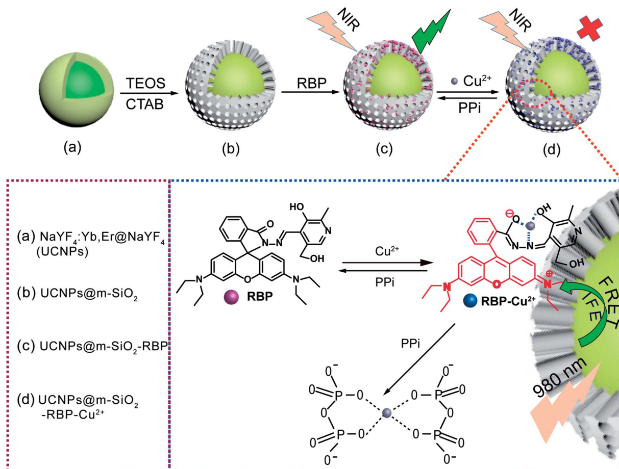
Scheme 1 Schematic of the detection of \text{Cu}^{2+} and PPI by RBP attached with UCNP. (a) Core-shell UCNP (b) UCNP@m-SiO 2 (c) UCNP@m-SiO 2 absorbed the RBP to form the composite probe (d) composite probe with \text{Cu}^{2+} .
